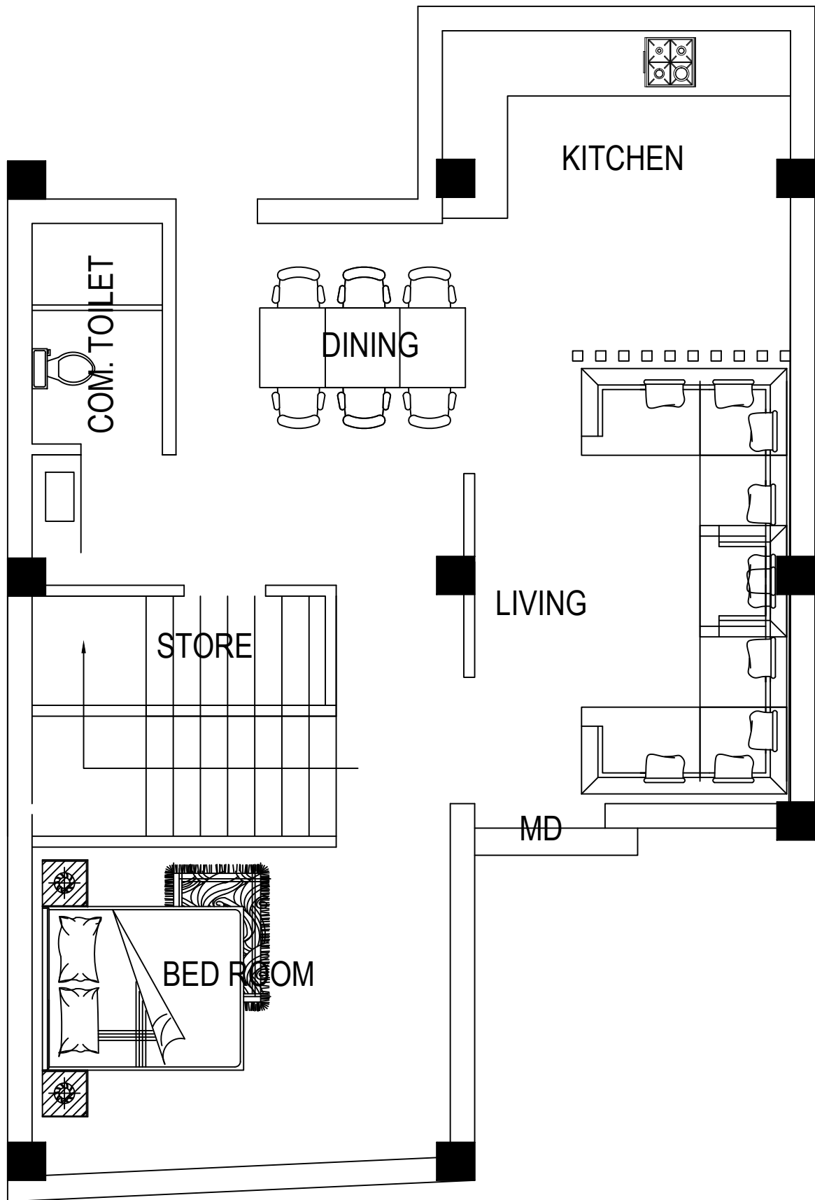
GROUND FLOOR PLAN AREA: 728 SQ.FT
